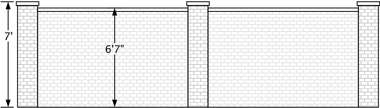
Brick wall 16" columns every approx. 10'
