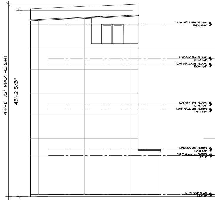
LEFT-WEST ELEVATION
