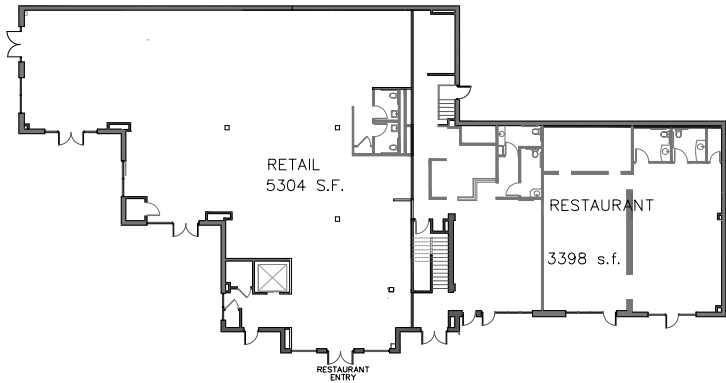
○ GROUND FLOOR PLAN 3/32"=1'-0"
