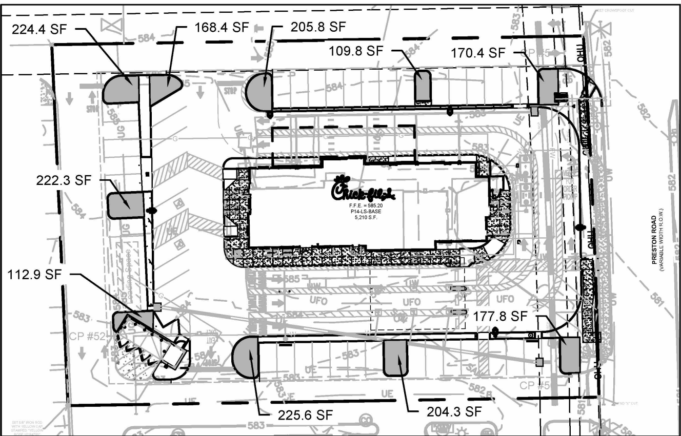
LANDSCAPE ISLANDS SCALE 1:50
