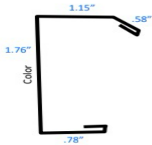
Snap in Base
