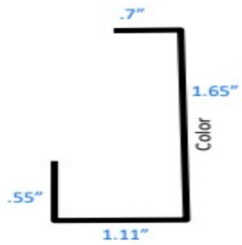
Snap in Channel
