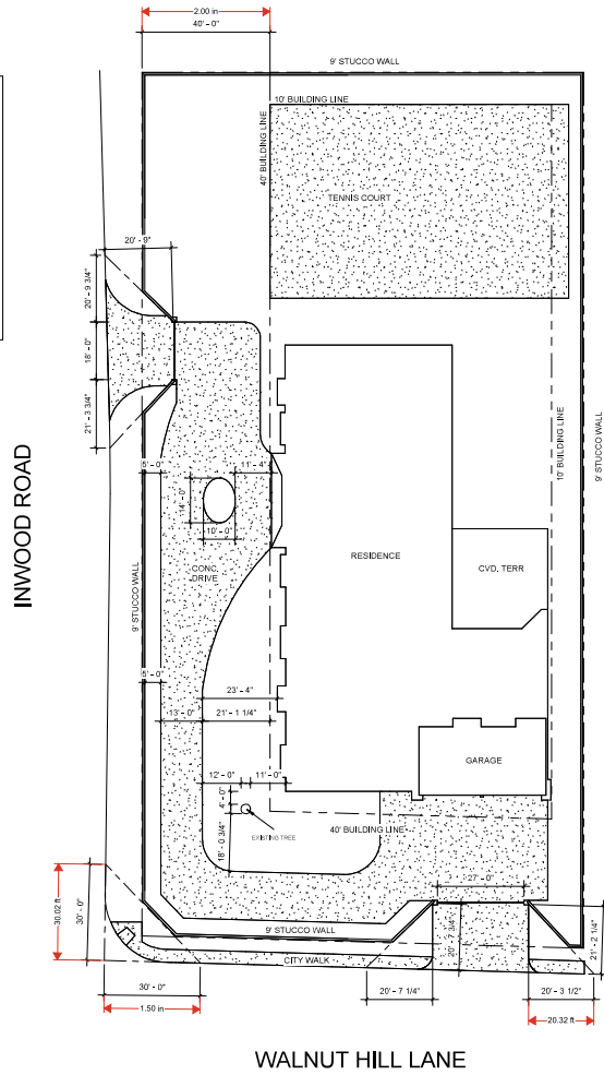
1 SITE PLAN 1" = 20'-0"
