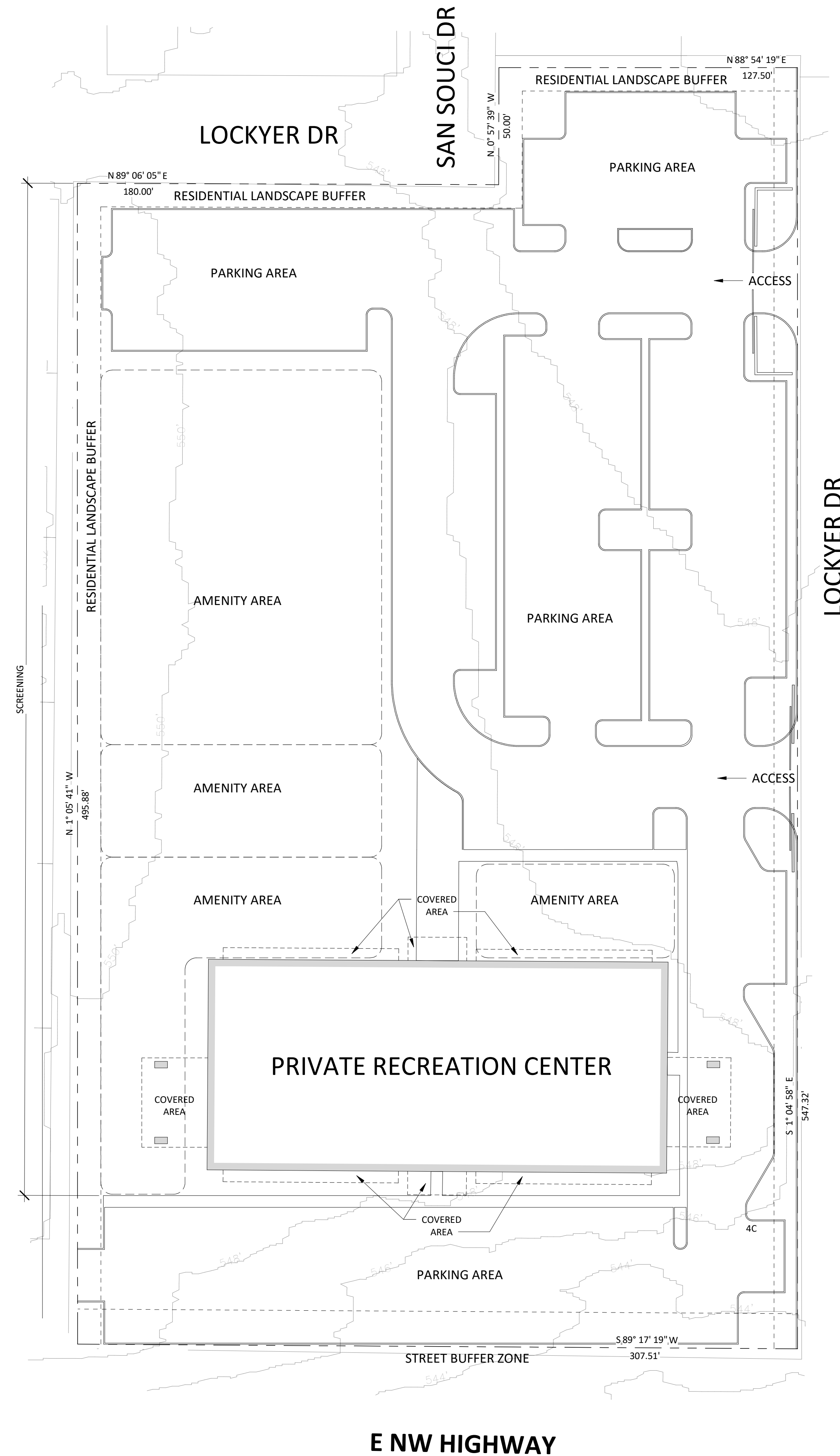
1 CONCEPTUAL PLAN 1" = 30'-0"
