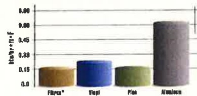
Thermal Conductivity
