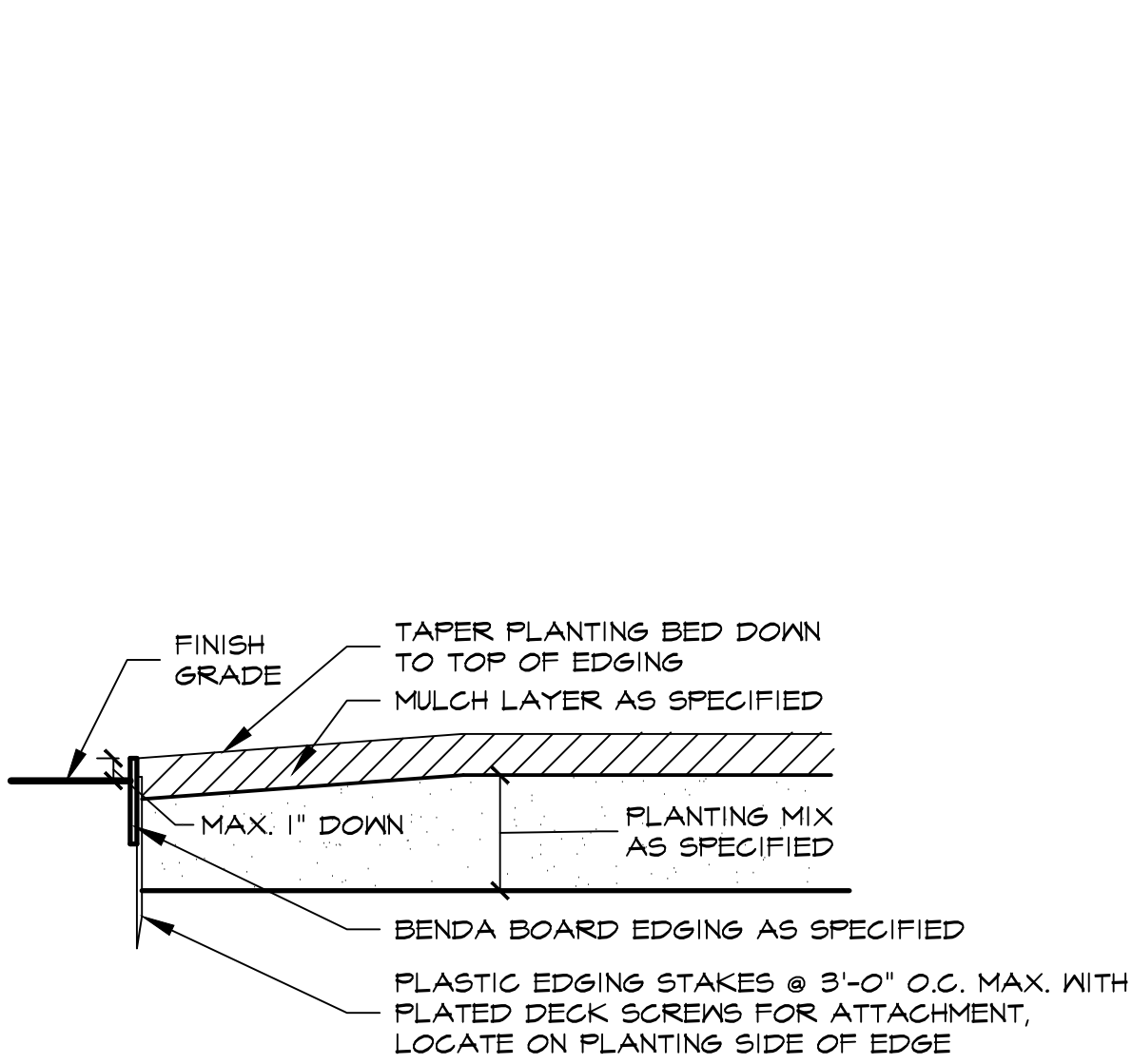
3 TYPICAL BED EDGING DETAIL NOT TO SCALE
