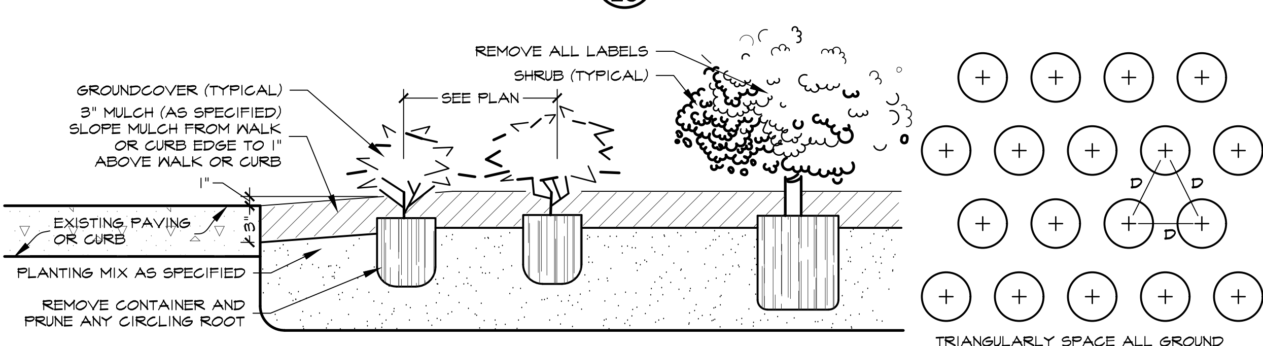
2 SHRUB AND GROUND COVER PLANTING DETAIL NOT TO SCALE
