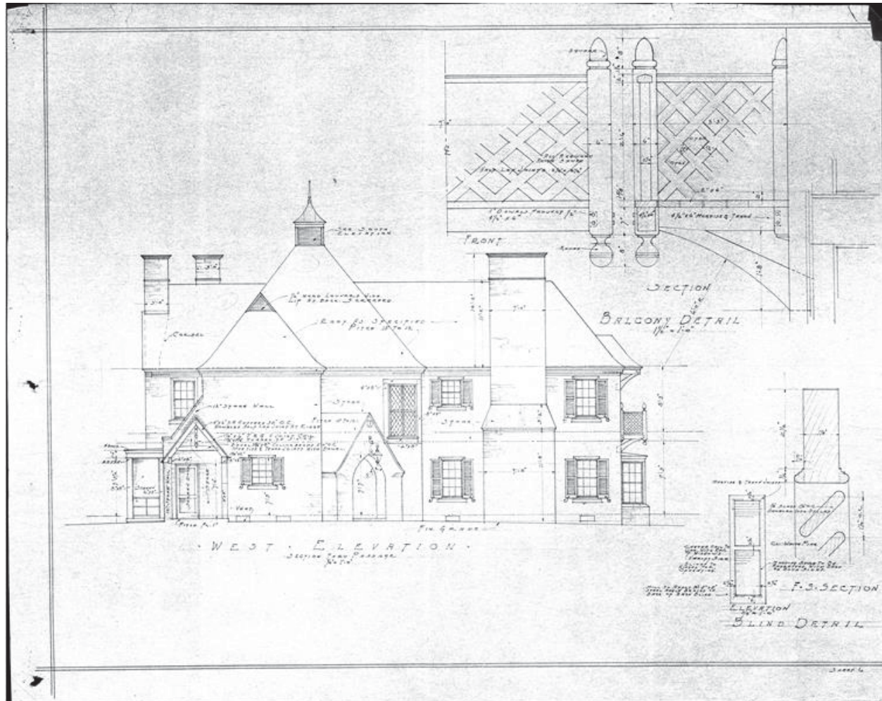
West Elevation
