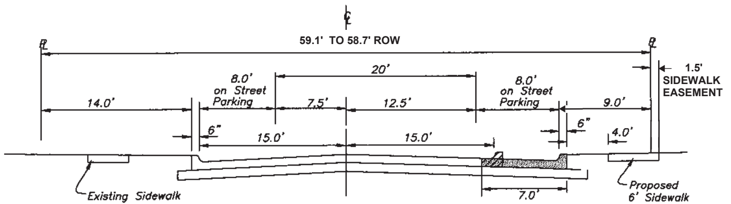
COCKRELL TYPICAL PAVEMENT SECTION
