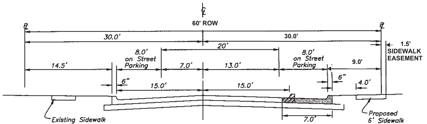
MCKEE TYPICAL PAVEMENT SECTION
