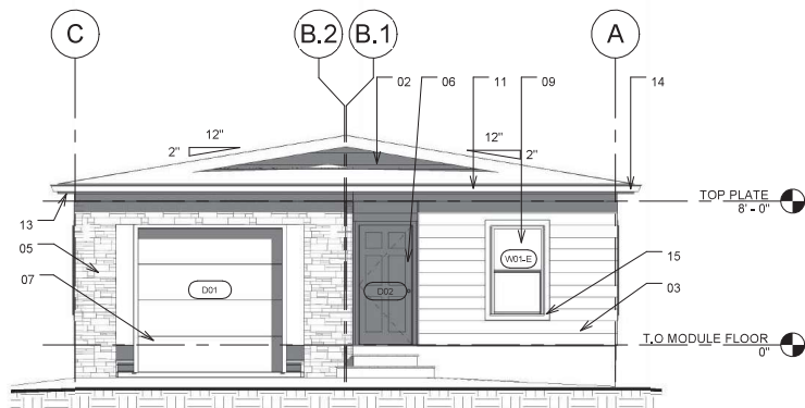
① Type B - Front Elevation 3/16" = 1'-0"
