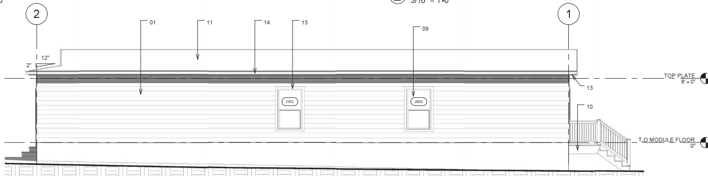
① Type B - Front Elevation 3/16" = 1'-0"
