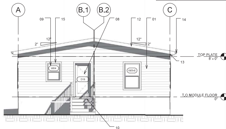
② Type B - Rear Elevation 3/16" = 1'-0"
