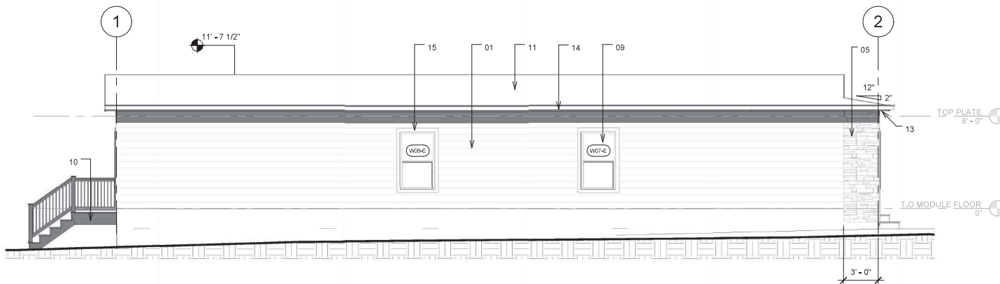
④ Type B - Left Side Elevation 3/16" = 1'-0"
